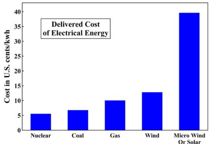
Figure 26: Delivered cost per kilowatt hour of electrical energy in Great Britain in 2006, without CO 2 controls (126). These estimates include all capital and operational expenses for a period of 50 years. Micro wind or solar are units installed for individual homes.
